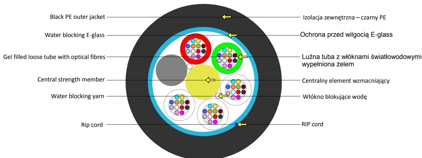
The picture represents a cable with 60 fibres
